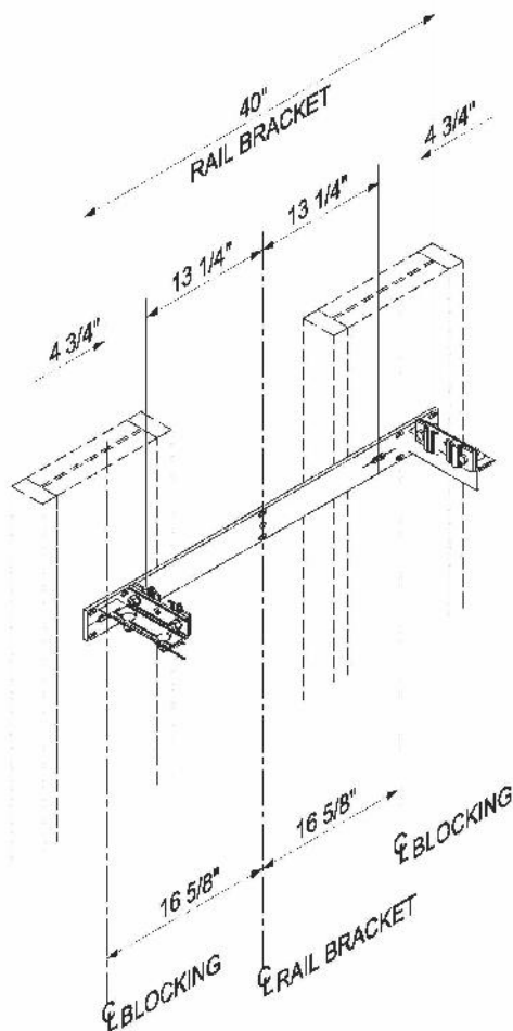
Wood Blocking Guidelines
